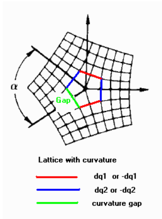
Disclination gap due to curvature.
