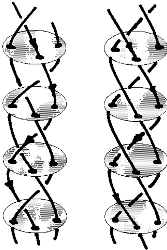
Spin 0 (Chaotic)
