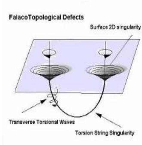
Figure 2. Falaco Topological Defects.
