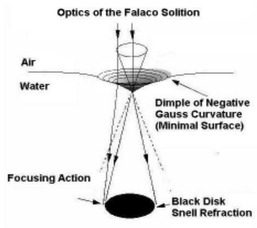
Figure 1. Optics of the Falaco Soliton
