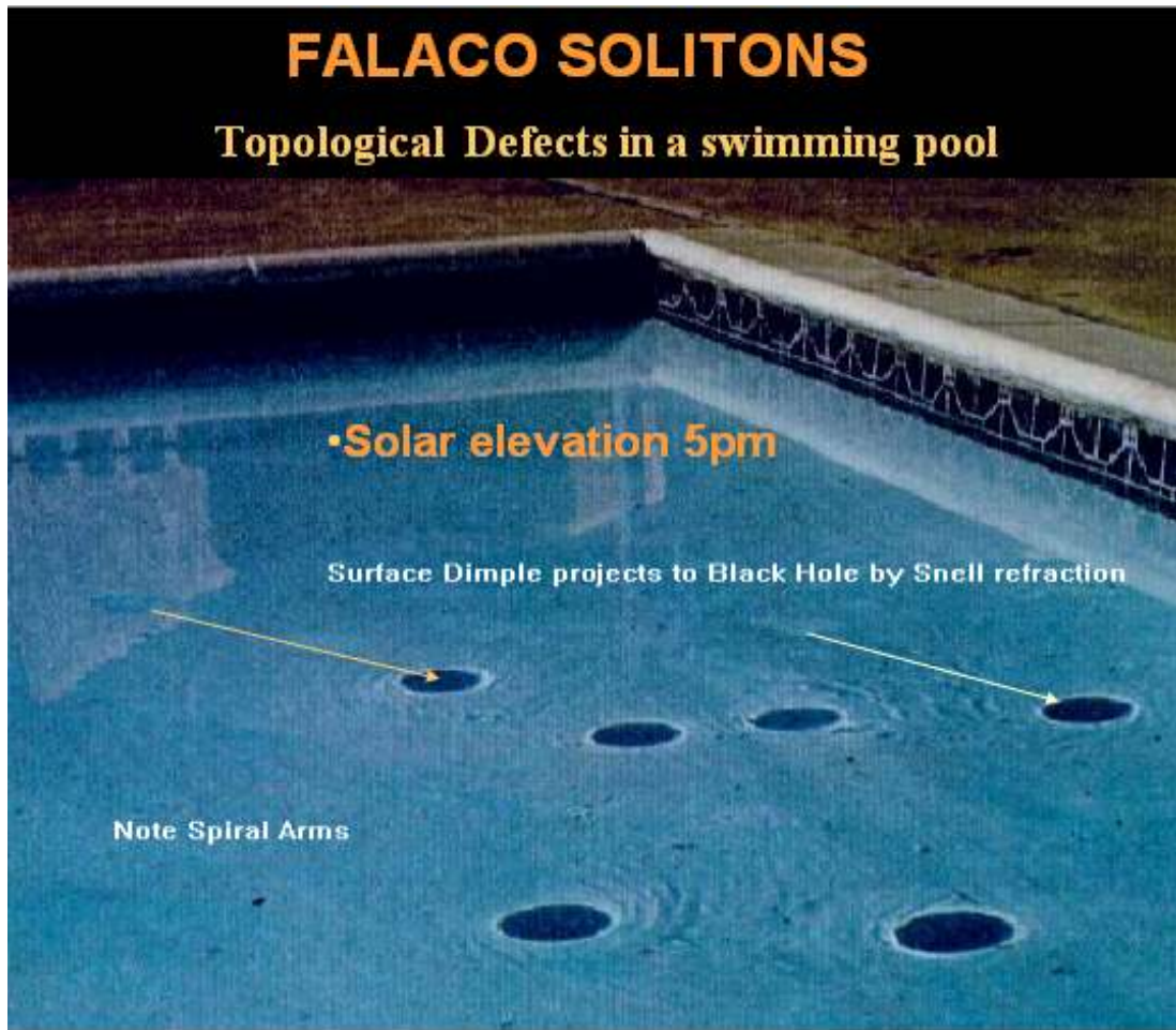
Figure 1. Three pairs of FALACO SOLITONS, a few minutes after creation. The kinetic energy and the angular momentum of a pair of
